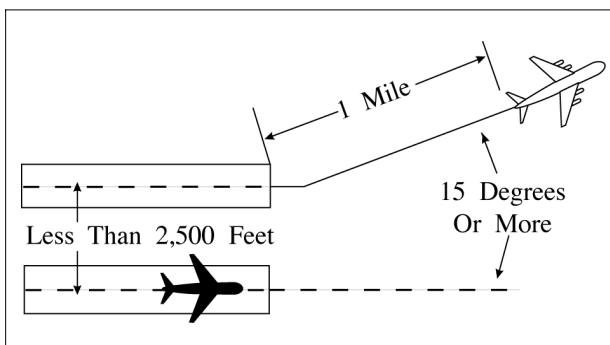
FIG 5-8-2 Simultaneous Departures
