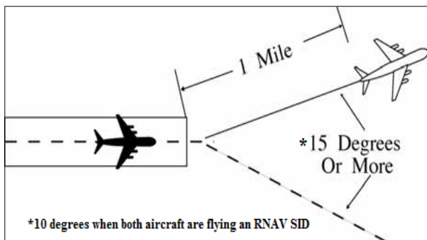
FIG 5-8-1 Successive Departures
