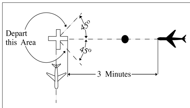
FIG 6-3-1 Separation Minima
