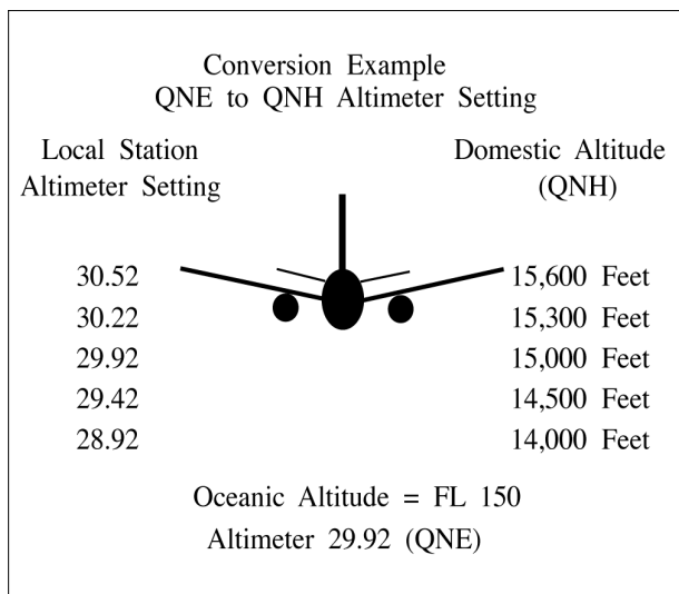
FIG 8-5-1
