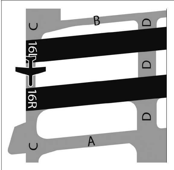
FIG 3-9-21 Runway/Taxiway Proximity
