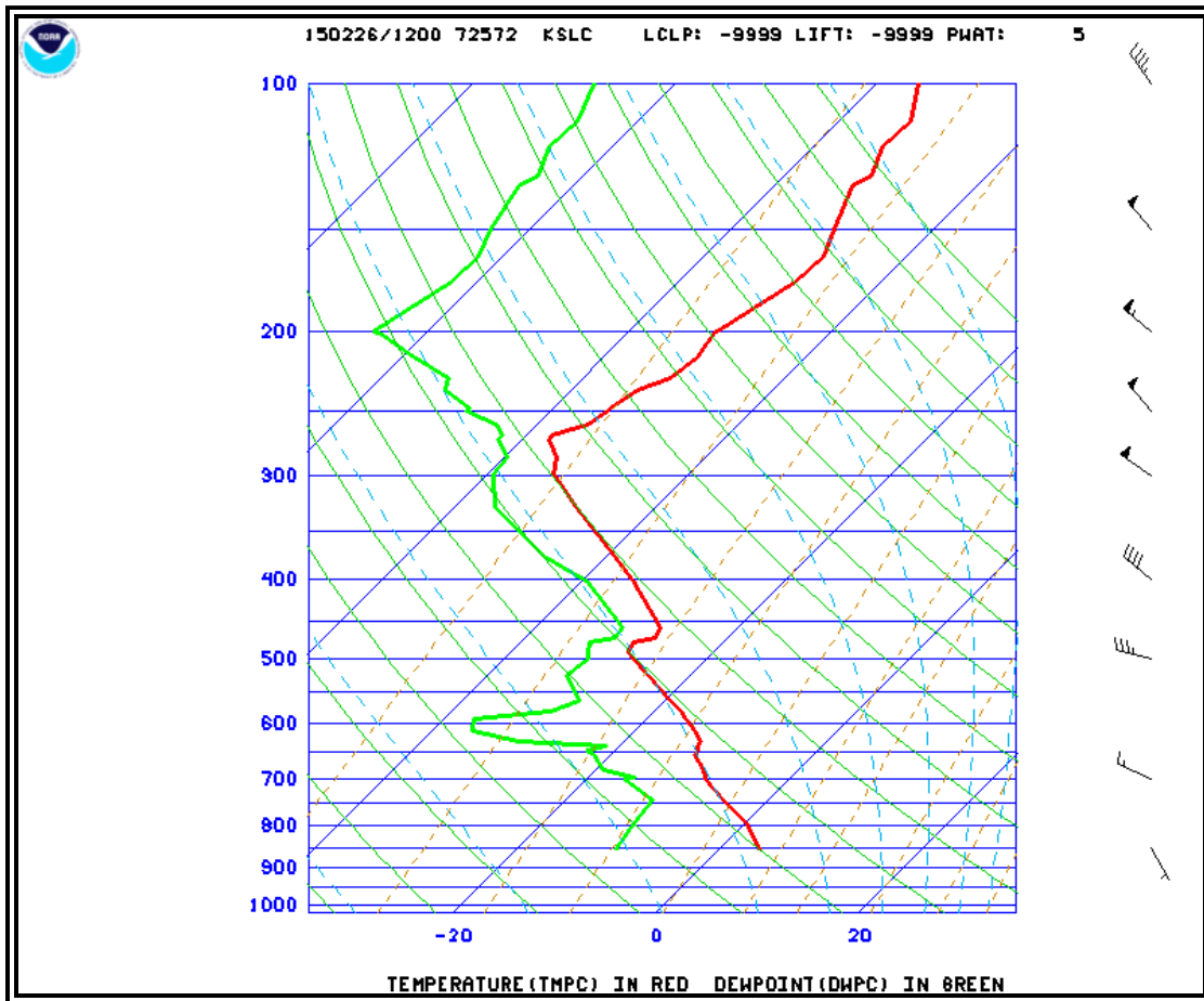
Figure 4-22. Skew-T Diagram—Example
