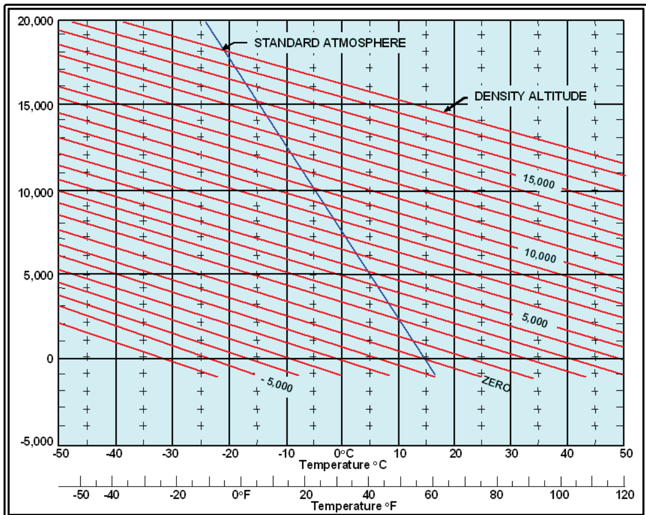
Figure C-1. Density Altitude Computation Chart
