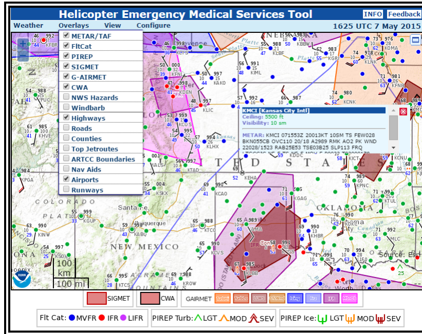
Figure 6-11. HEMS Data Overlays with Text METAR—Example
