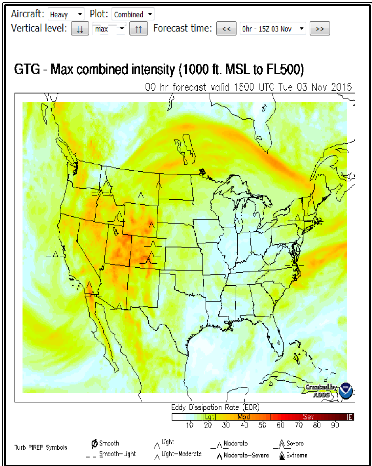
Figure 5-75. GTG—Max Intensity Example CAT+MWT All Levels
