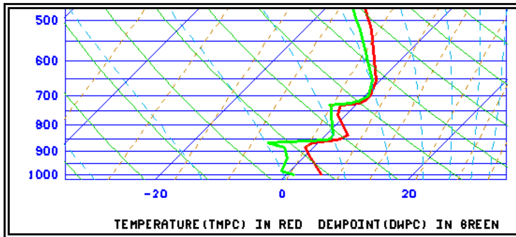
Figure 4-23. Skew-T Diagram—Multiple Freezing Level Example
