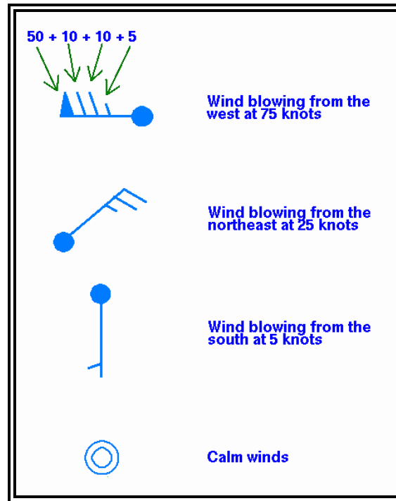
Figure 4-8. NWS Surface Analysis Chart Wind Plotting Model
