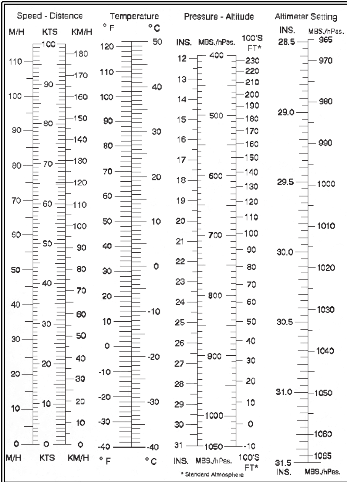
Figure B-1. Standard Conversion Chart
