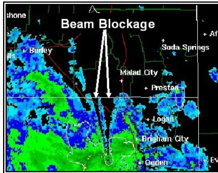
Figure 3-21. WSR-88D Weather Radar Beam Blockage on Base Reflectivity Product Example
