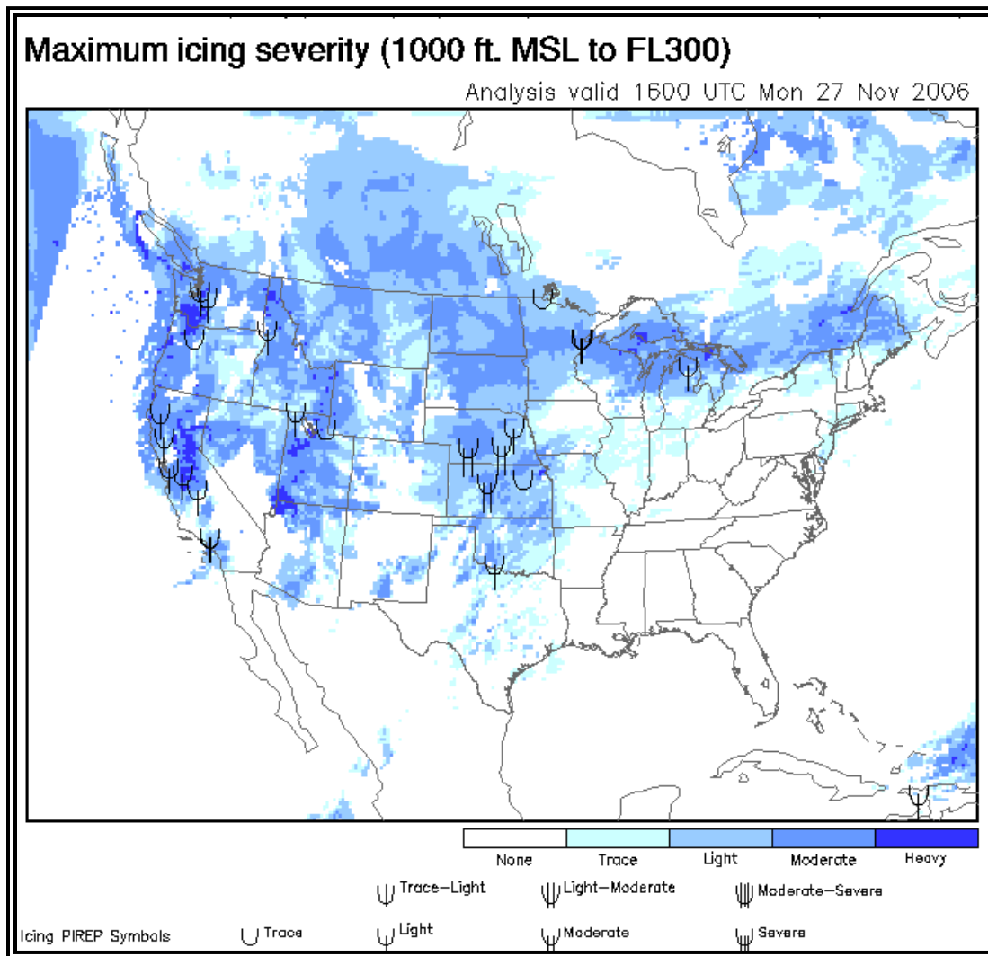
Figure 5-72. CIP/FIP Icing Severity—Max Example
