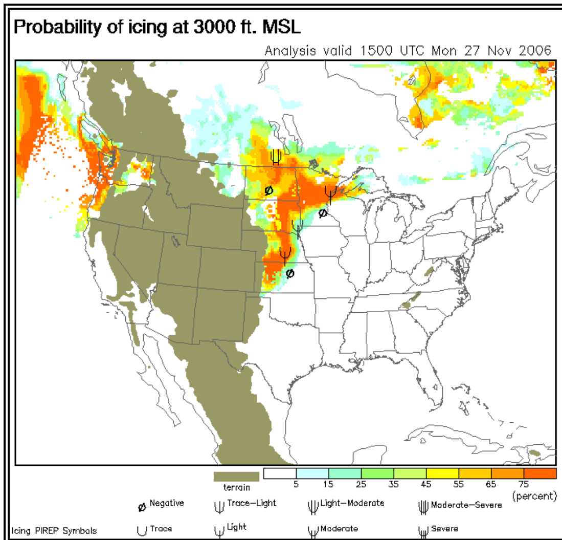
Figure 5-69. CIP/FIP Icing Probability (3,000 Feet MSL)—Example
