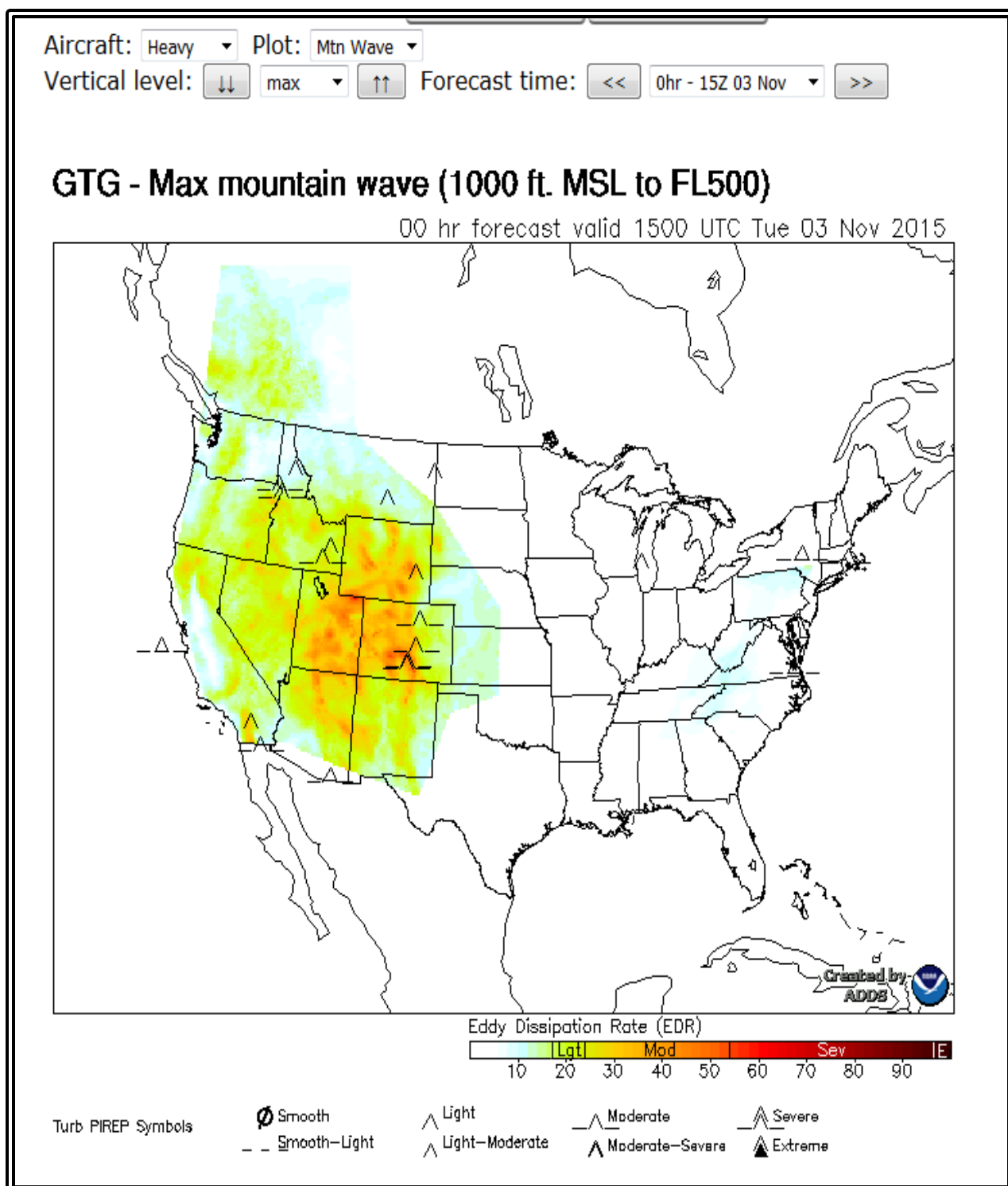
Figure 5-77. Explicit MWT Forecasts Example
