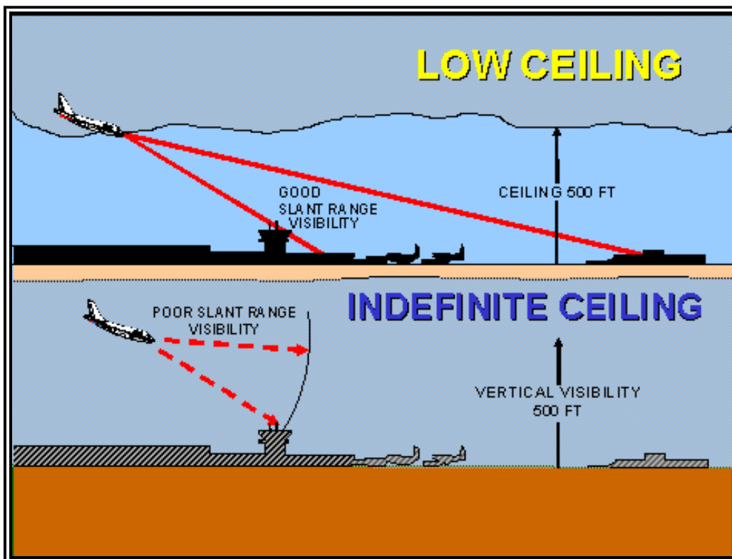
Figure 3-3. Obscuration Effects on Slant Range Visibility
