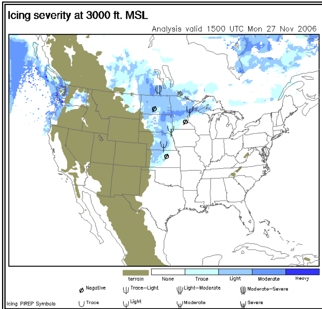
Figure 5-71. CIP/FIP Icing Severity (3,000 Feet MSL)—Example
