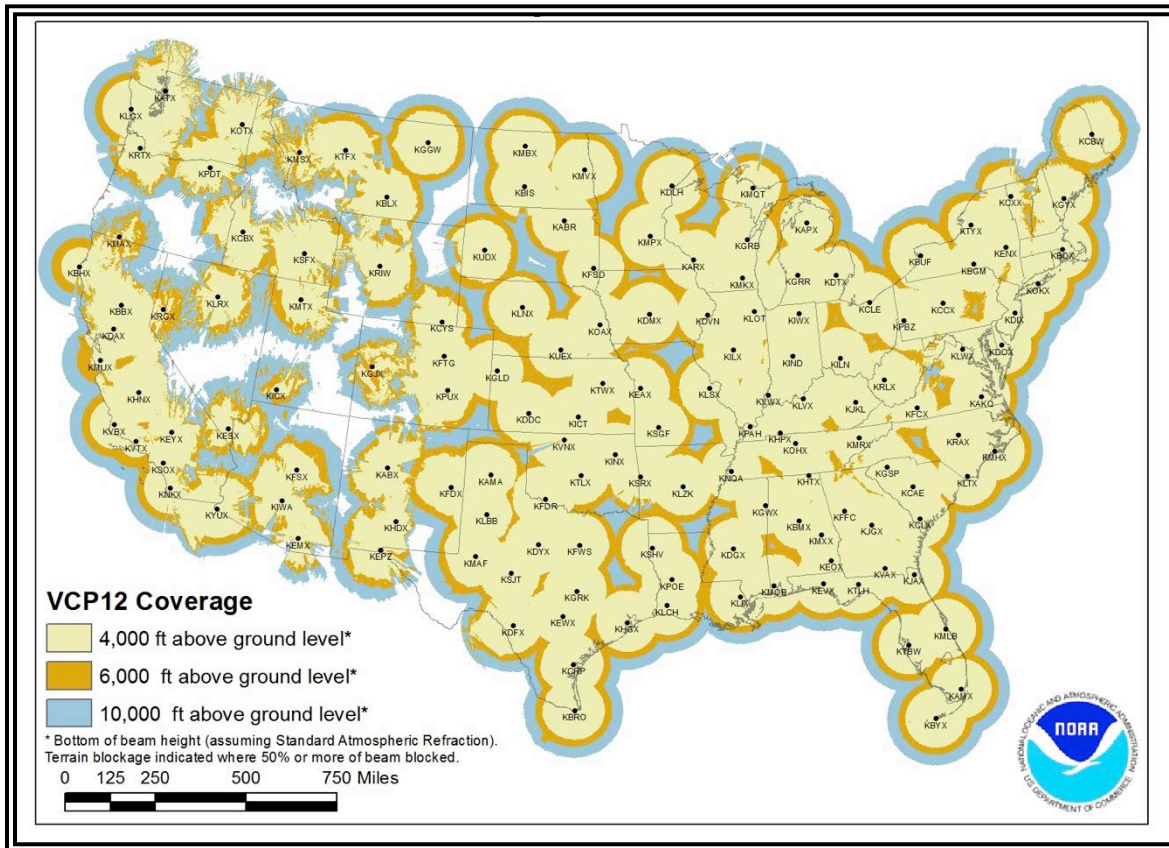
Figure 3-6. Location of WSR-88D Weather Radar in the CONUS and Their Respective Coverage at 4,000 Feet AGL, 6,000 Feet AGL, and 10,000 Feet AGL
