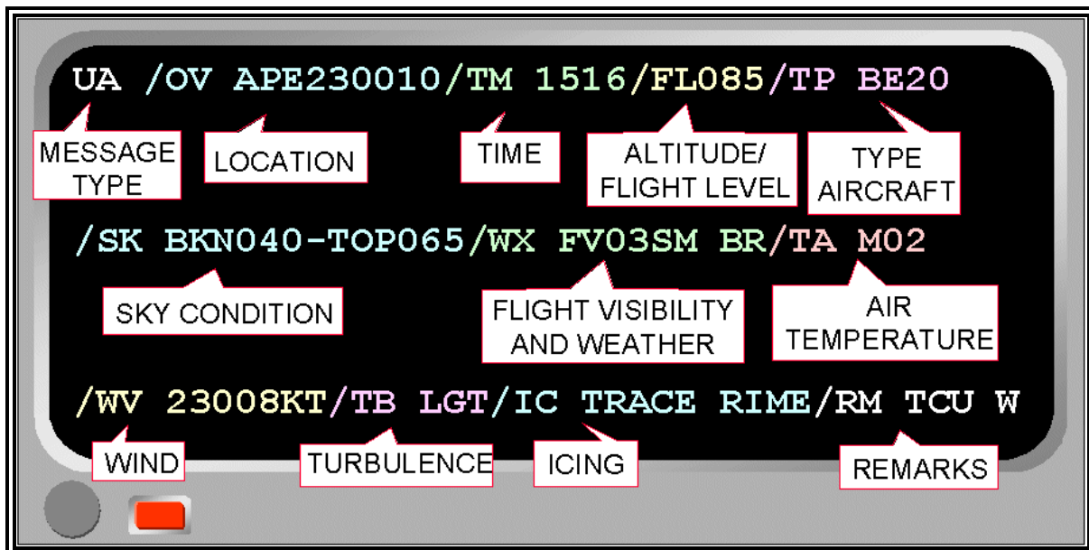
Figure 3-5. Pilot Weather Report (PIREP) Coding Format
