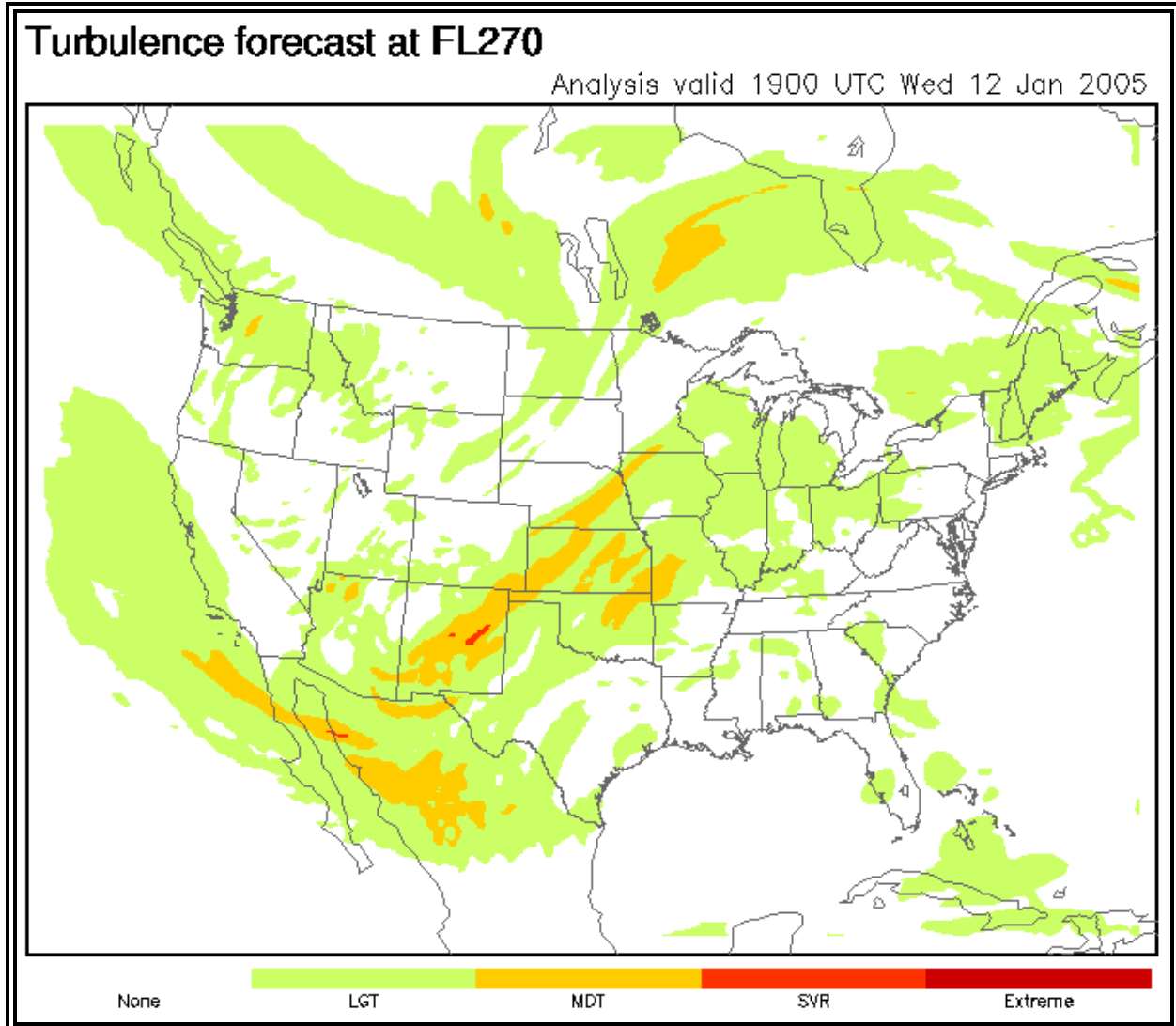
Figure 9-23. GTG Example
