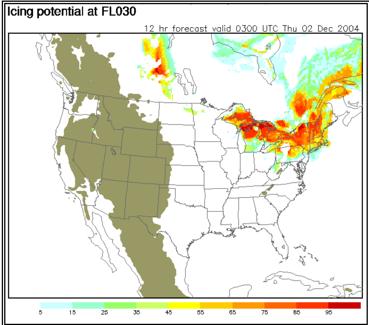
Figure 9-22. FIP Example
